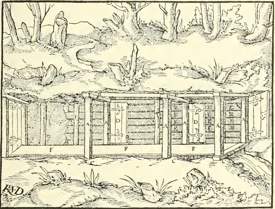
A—POSTS. B—CAPS. C—SILLS. D—DOORS. E—LAGGING. F—DRAINS.
